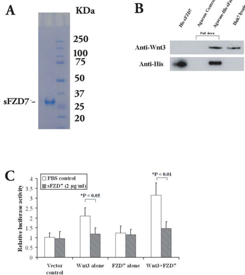
Figure 1 sFZD7 binds to Wnt3 and suppresses Wnt3-induced \beta -catenin/Tcf4 transcriptional activation in Huh7 cells. (A) SDS-PAGE analysis of purified sFZD7. (B) Pull-down assay demonstrating the interaction between sFZD7 and Wnt3. Huh7 cells lysate was pulled down with Ni-NTA agarose with or without recombinant His-sFZD7 peptide. Protein complexes were centrifuged and eluted, and the supernatants analyzed by Western blot using rabbit anti-Wnt3 antibody (upper panel) and anti-His antibody (lower panel). Huh7 lysate and recombinant His-sFZD7 were used as positive controls. (C) sFZD7 abolished the Wnt3-induced \beta -catenin/Tcf4 transcriptional activity in Huh7 cells. Huh7 cells were transfected with 0.2 \mu g of each of the indicated expression plasmid, along with 0.3 \mu g of pTOPFLASH or pFOPFLASH reporter plasmids and 0.1 \mu g of \beta -gal to normalize for transfection efficiency. The results are expressed as means \pm SD (error bars) of triplicate assays. *P < 0.05 versus control.
