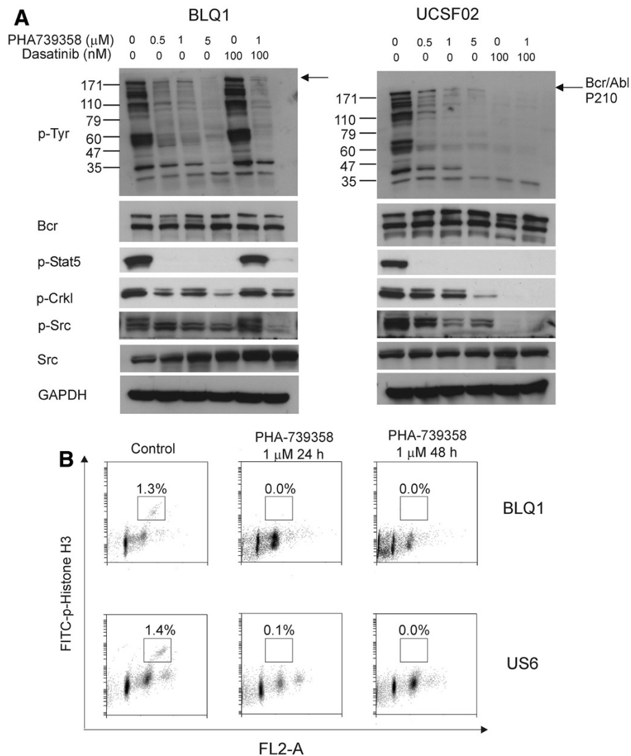
Figure 3 PHA-739358 eliminates activity of both Bcr/Abl and Aurora kinase. (A) BLQ1 (Ph-positive T315I mutation) and UCSF02 (Ph-positive no mutation) cells were incubated with the indicated concentrations of PHA-739358 with or without dasatinib (100 nM) for 24 hours. Phosphorylation status of Bcr/Abl, Stat5, Crkl and Src was assessed by Western blot. Blots were stripped and reprobbed with Bcr, Src and Gapdh as loading controls. (B) BLQ1 and US6 cells were exposed to 1 μM PHA-739358 for 24 and 48 hours and the percentage of phospho-histone H3 (Ser10) positive cells was defined by flow cytometry.
